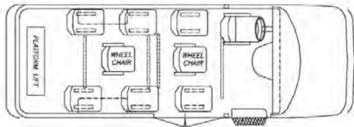
7 Passenger Seating with 2 Wheelchair Positions
