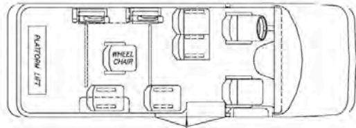
10 Passenger Seating or 6 Passenger with 1 Wheelchair
