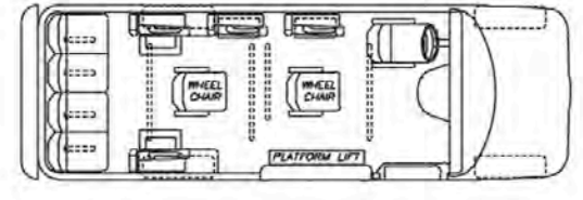
11 Passenger Seating with 2 Wheelchair Positions
